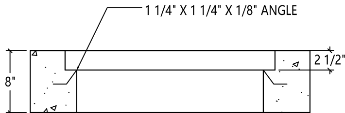
SECTION VIEW
