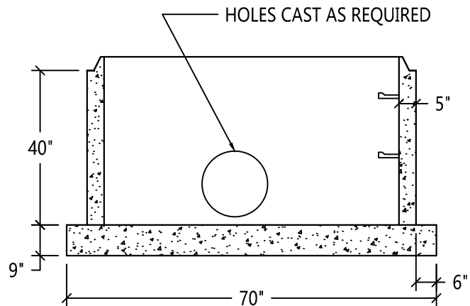
BASE SECTION
