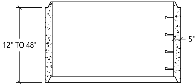
RISER SECTION
