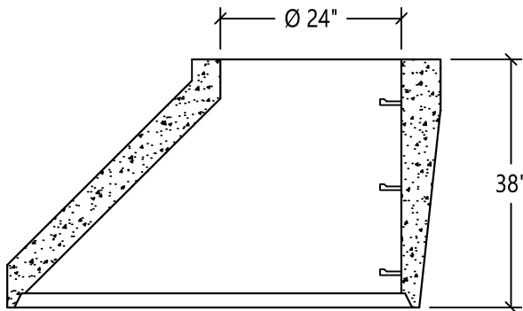
CONE SECTION
