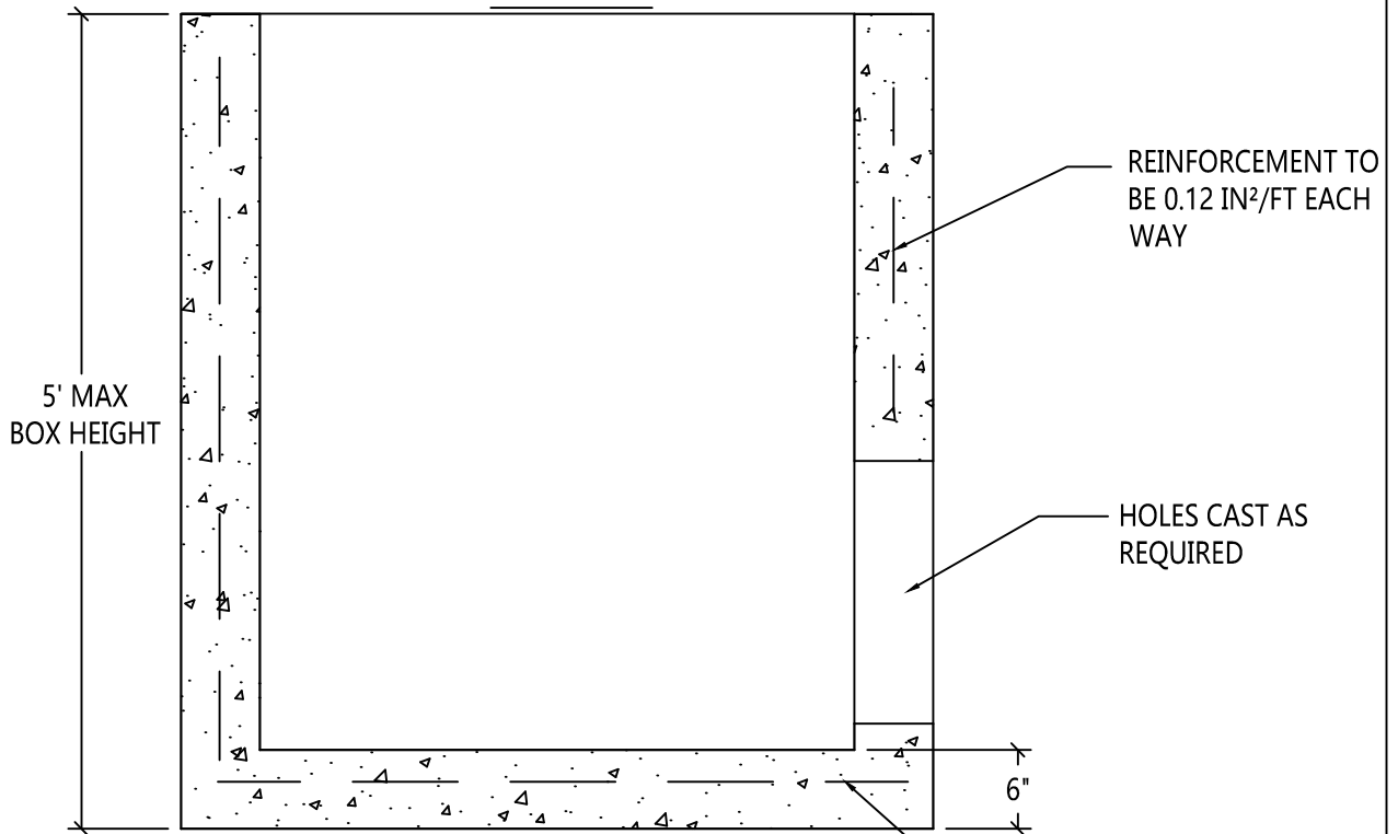
SECTION VIEW
