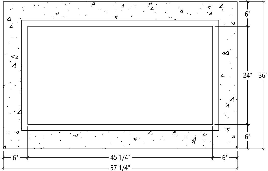
PLAN VIEW
