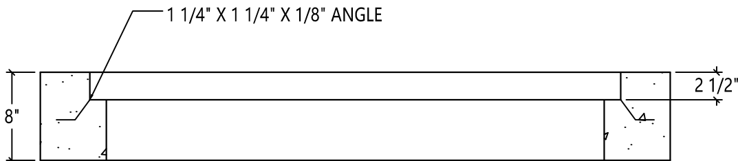
SECTION VIEW
