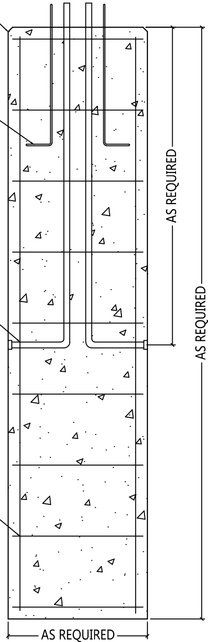
TYPICAL ELEVATION
